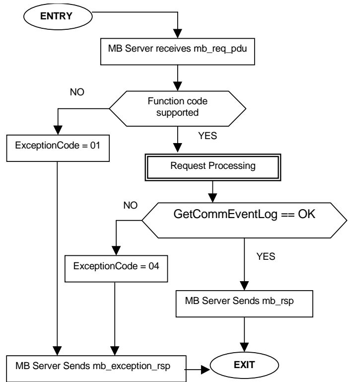
Figure 20: Get Comm Event Log state diagram
